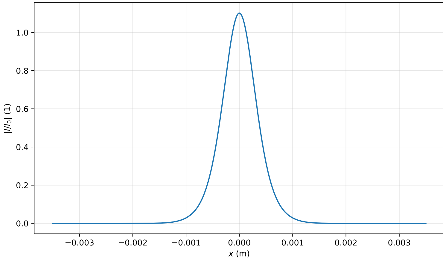
Intensity profile I(x, y = 0, z = 1.274m)/I_0 , P_{in}=0.6P_{cr} , artificial time
